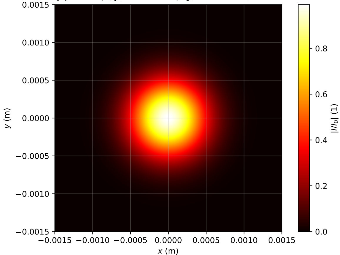
Intensity profile I(x, y, z = 0.239m)/I_0 , Pin=0.1Pcr, artificial time
